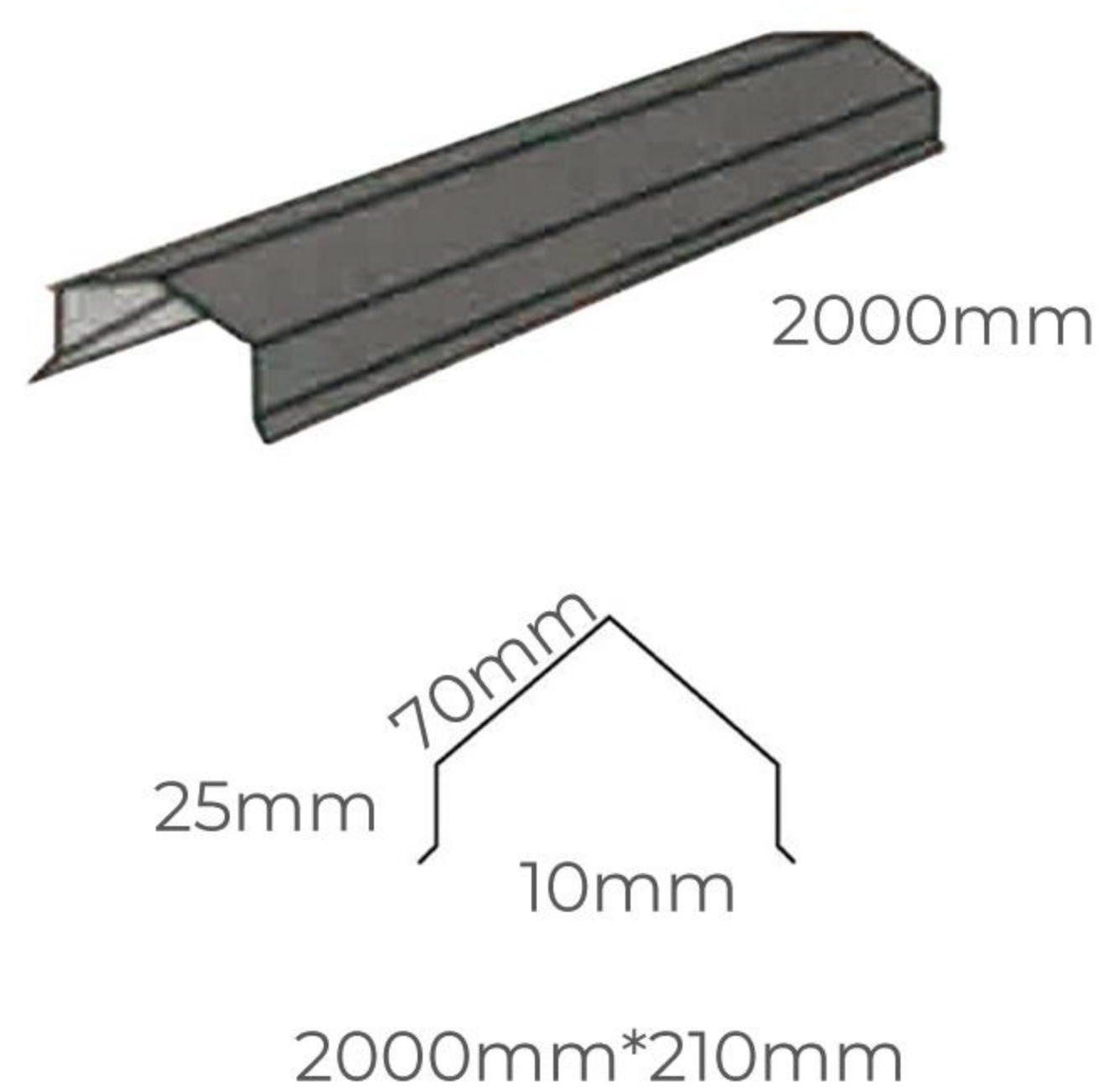
2. Angle Ridge Cap 2
