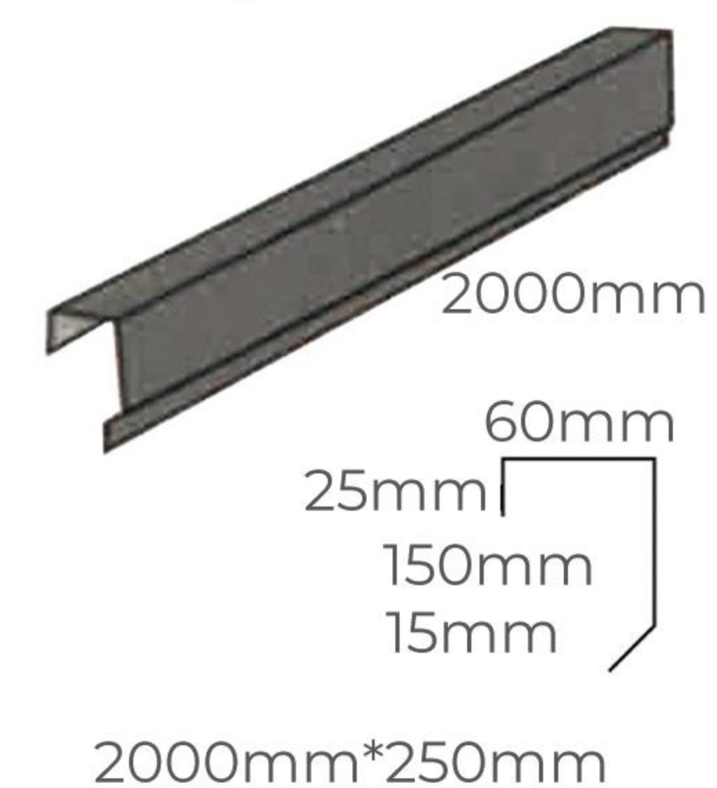
7. Barge Board Cover
