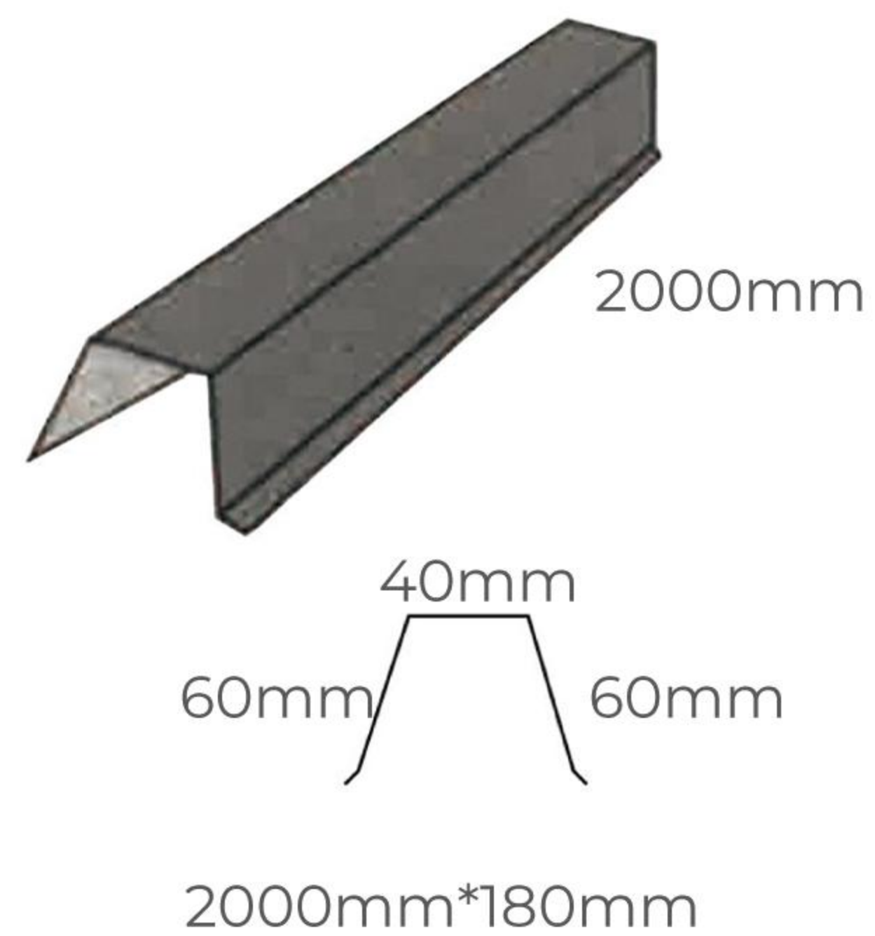
3. Square Ridge Cap
