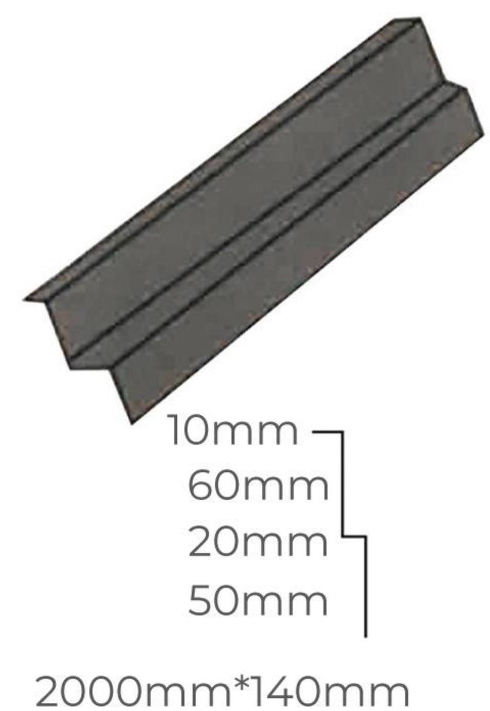
4. Wall Side Flashing
